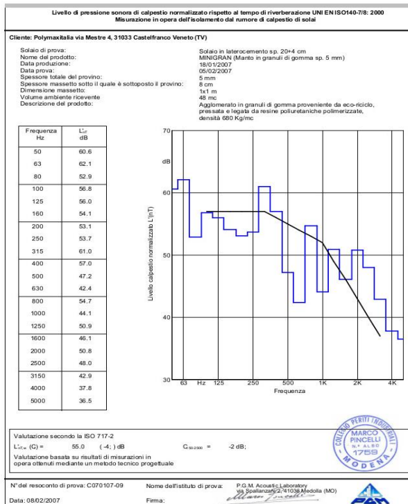
Gráfico 3: L st,w MINIGRAN sp. 5 mm - massetto sp. 8 cm
