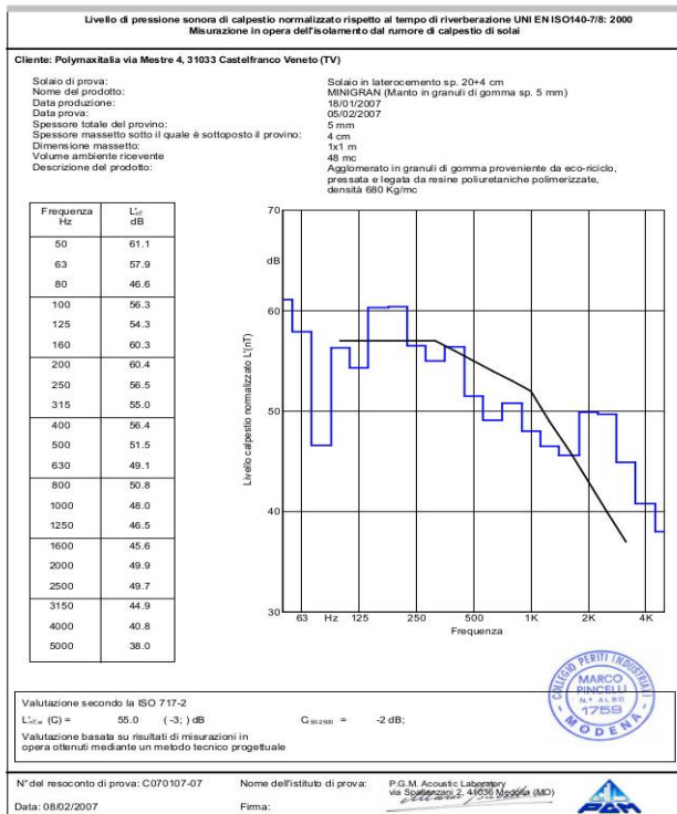
Gráfico 1: L st,w MINIGRAN sp. 5 mm - massetto sp. 4 cm
