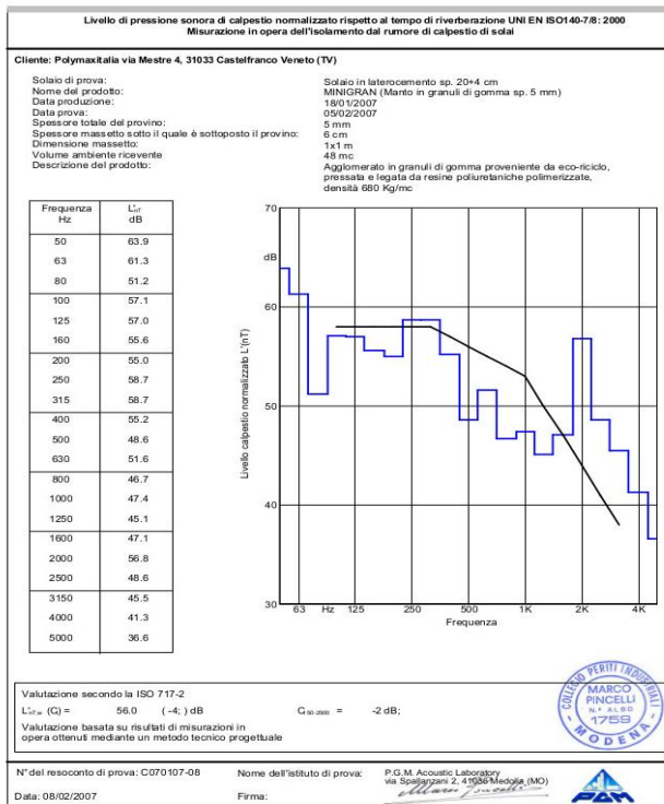
Gráfico 2: L st,w MINIGRAN sp. 5 mm - massetto sp. 6 cm
